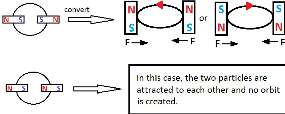
Fig.10 placing two magnetic particles in a circuit so that the velocity vector and the magnetic field are on a horizontal plane
