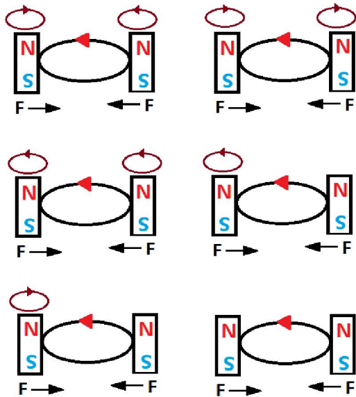
Fig.8 six states that can be six anti-quark structures in the direction of B
