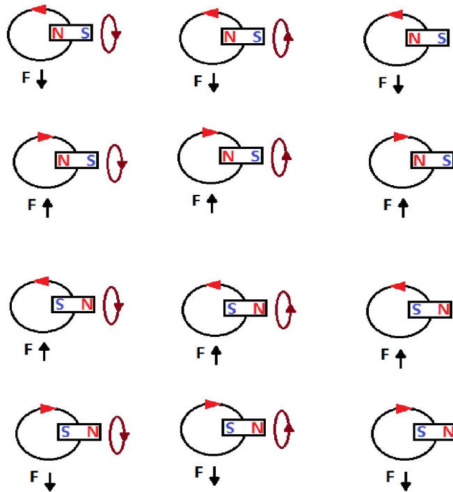
Fig.9 Twelve modes of gauge bosons
