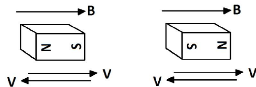
Fig.4 this kind of particle motion is impossible
