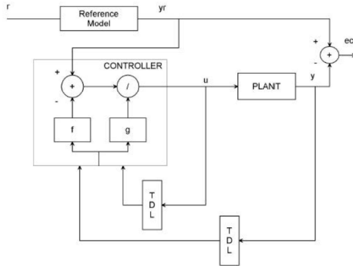
Figure 2 NARMA-L2 Controller.
