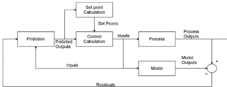
Figure 3 Block diagram for model predictive control.
