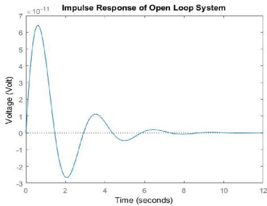
Figure 4 Open loop response
