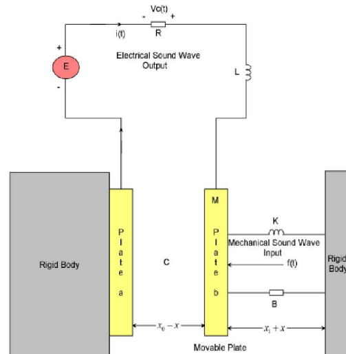
Figure 1 Capacitor microphone system
