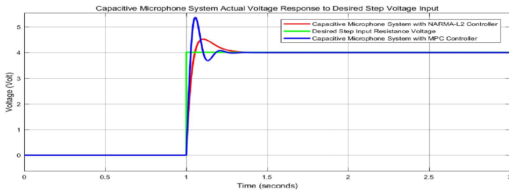
Figure 6 Step response simulation result
