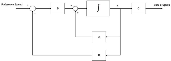
Figure 3 car mirror wiper system with robust pole placement method
