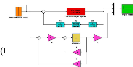
Figure 4 Simulink model of the vehicle windshield wiper system using H infinity Loop Shaping and
