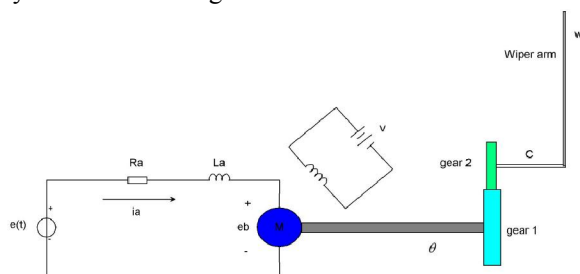
Figure 1 Electromechanical car mirror wiper system
