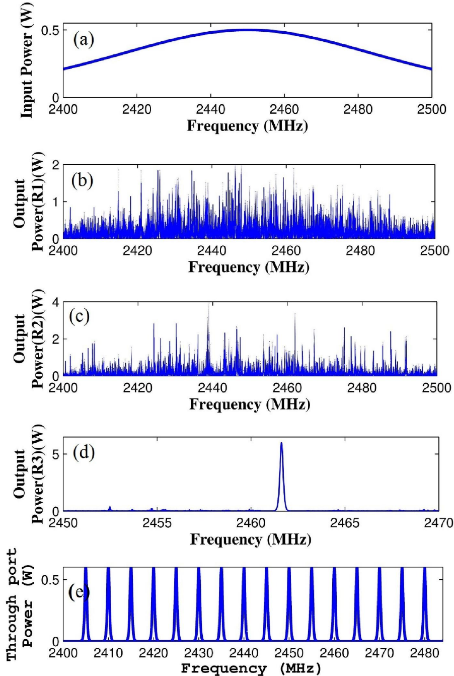
Figure 2: Discrete frequency generation steps for WSN using ZigBee, (a): Input Gaussian pulse, (b) Chaotic signals generated in ring 1, (c): Chaotic signal cancellation in ring 2, (d): Chaotic cancellation in ring 3, (e): discrete frequency channels generation.
