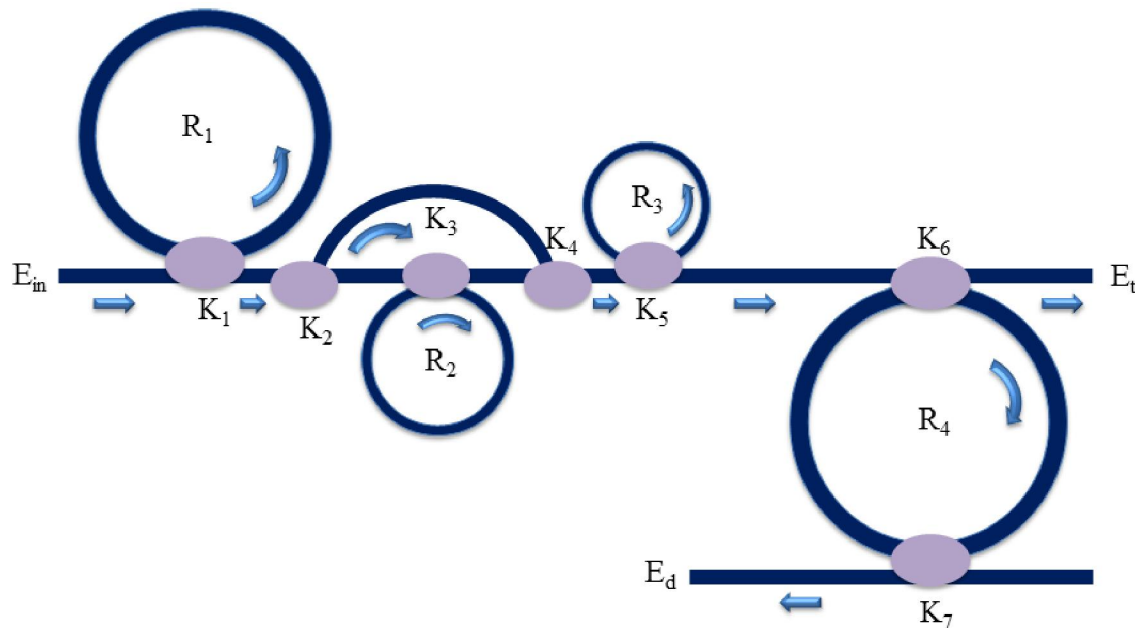
Figure 1. System of descrete frequency generation
