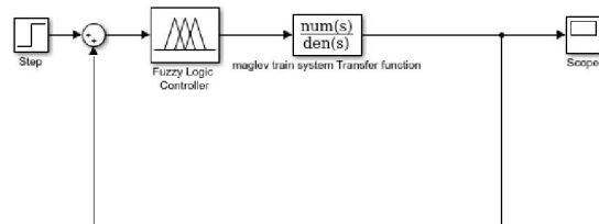
Fig 4. Simulink model of the fuzzy logic controller
