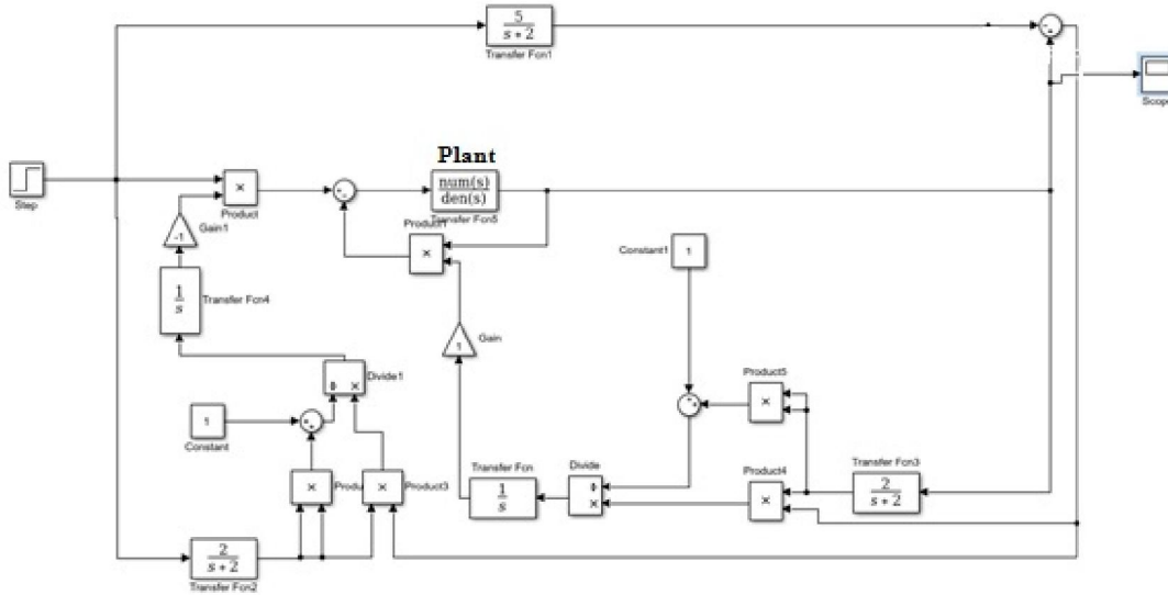
Fig 8 Simulink model of the Mras controller
