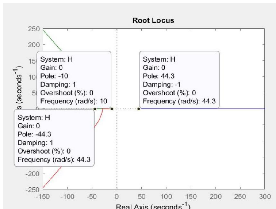
Fig 2. Root locus stability of maglev train system
