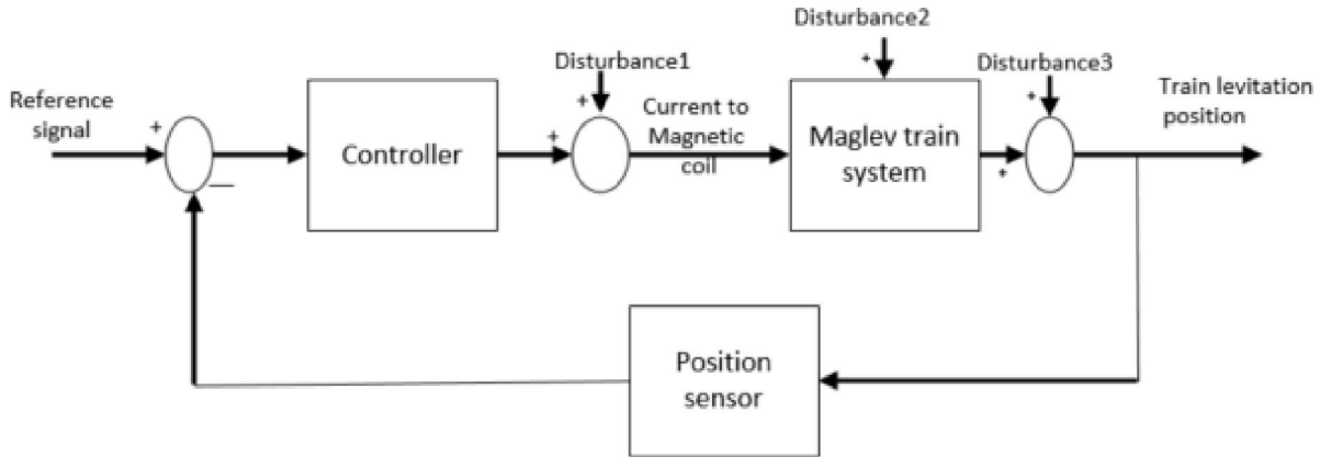
Fig 1. Block Diagram of Closed Loop Maglev Train Control System
