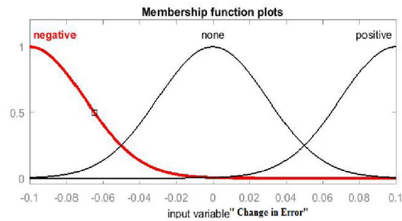
Fig 6. Change in error input
