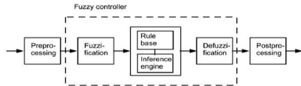
Fig 3. Block diagram of fuzzy logic Controller
