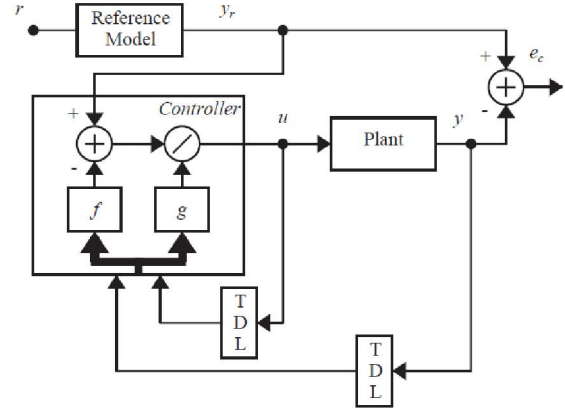
Figure 2 NARMA-L2 Controller.
