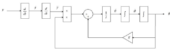
Figure 2 Block diagram of vertically moving base inverted pendulum
