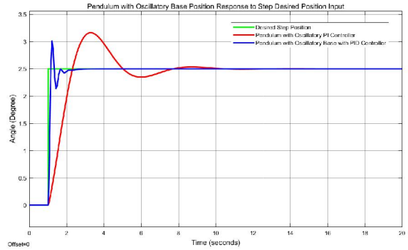
Figure 4 Step response simulation result
