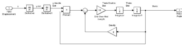
Figure 3 vertically moving base inverted pendulum subsystem
