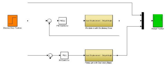
Figure 2 Simulink model of the vertically moving base inverted pendulum using PI and PID controllers for step input signal
