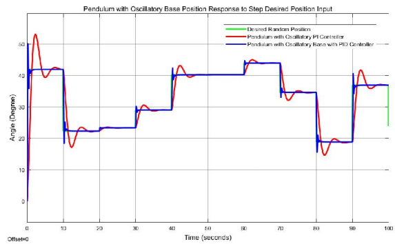
Figure 6 Random input signal simulation result
