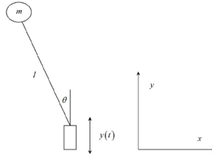
Figure 1 Vertically moving base inverted pendulum system
