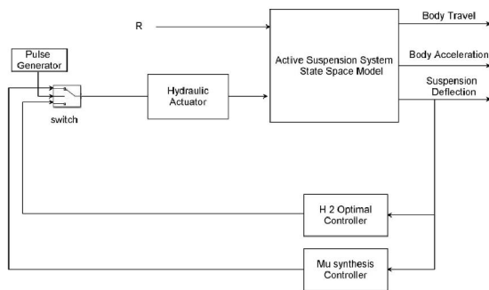
Figure 3: Active suspension system with H2 optimal and \mu -synthesis controller's system block diagram
