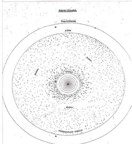
Atom is gigantic UNIVERSE having structure and properties exactly similar to the structure and properties resembling our Geo-UNIVERSE and Energy particle. Just as there are stars, planets, galaxies and life on the earth etc. present in the Geo-UNIVERSE, in the same way exactly similar: stars, planets, galaxies and life on Neutrons etc. may be present in the form of electrons, protons and neutrons in the atom.
