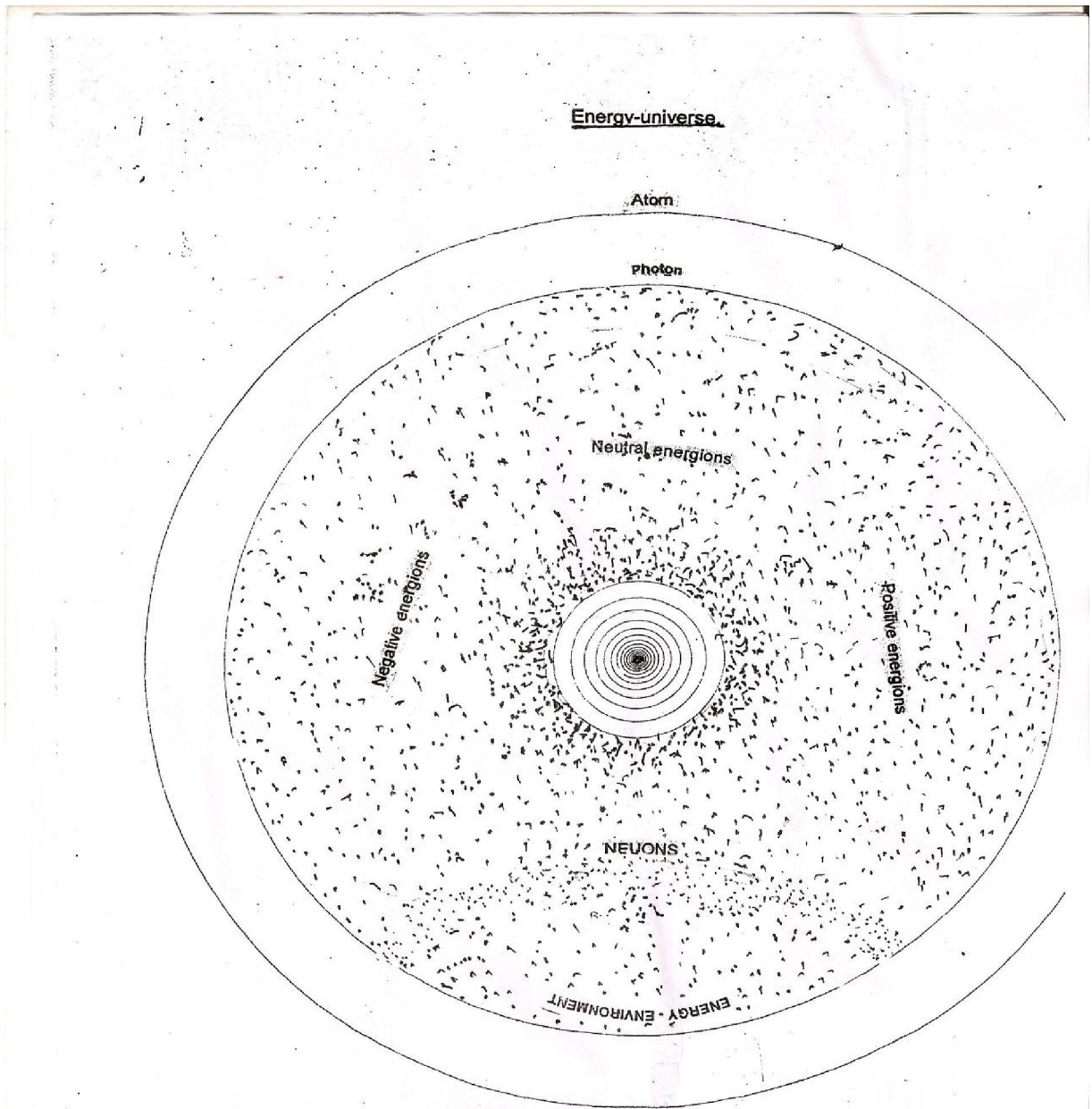
Energy particle has internal structure and having three kinds of basic elements proposed and named as Positive energions (PEONS) Negative energions (NEONS) and Neutral energions (NEUONS). It is also another universe named as Energy- Universe having structure and properties exactly similar to the structure and properties resembling our Geo- Universe and Atomic- Universe.
