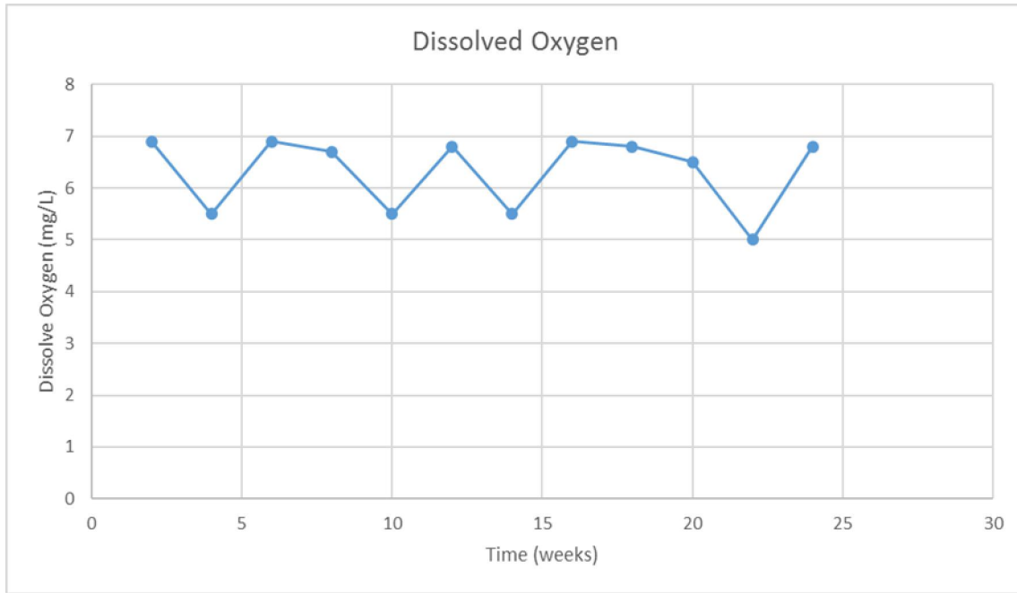
Figure 6: Average Dissolved Oxygen Measured in all Treatments
