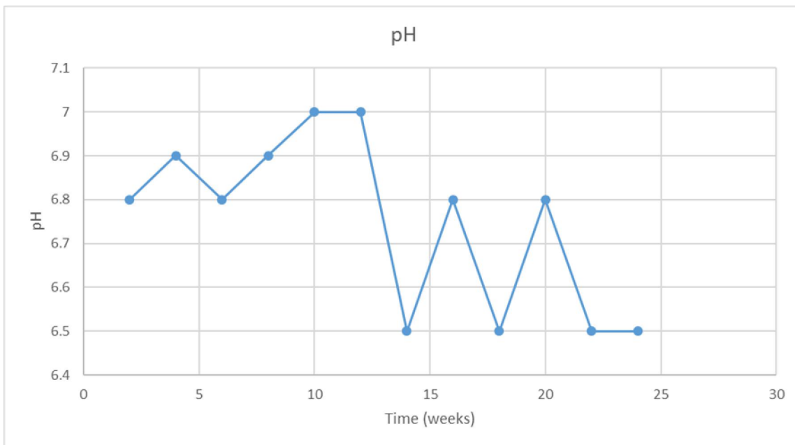
Figure 7: Average pH Measured in all Treatments
