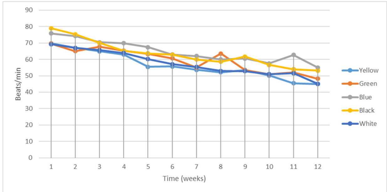
Figure 10: Mean Opercular Respiratory Rate (beats/min) in all Treatments measured fortnightly.
