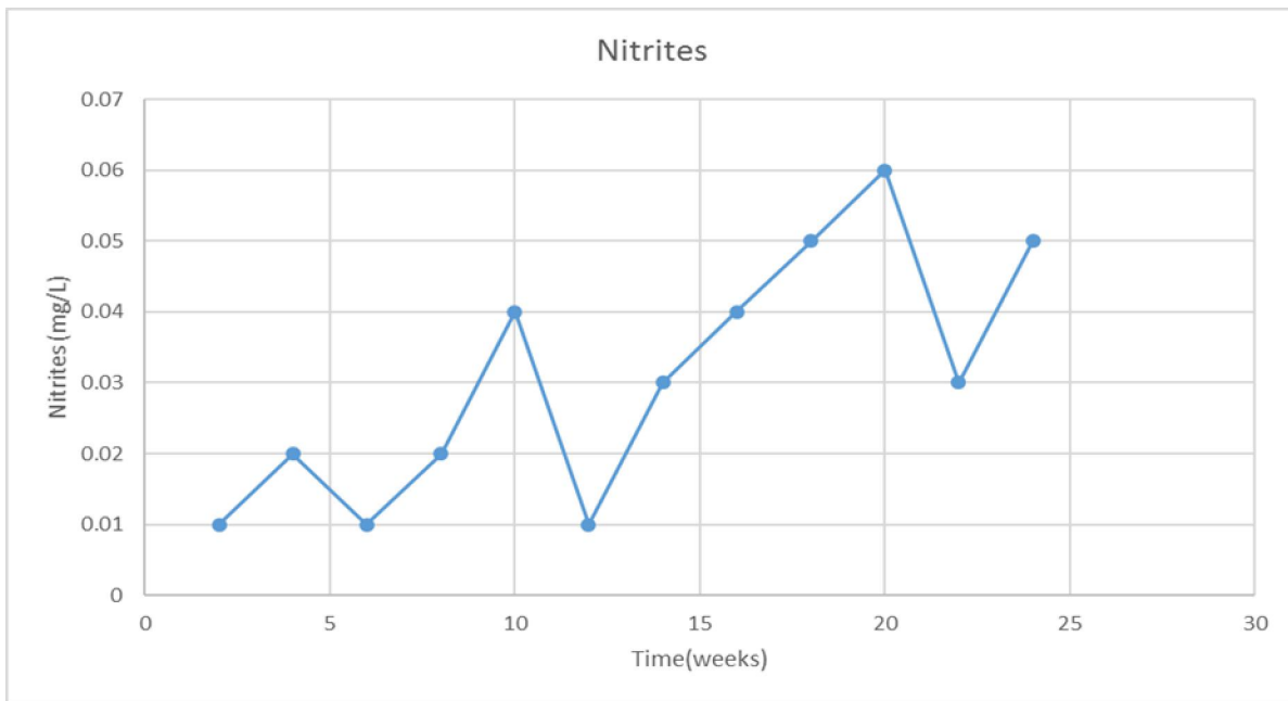
Figure 8: Average Nitrites Measured in all Treatments
