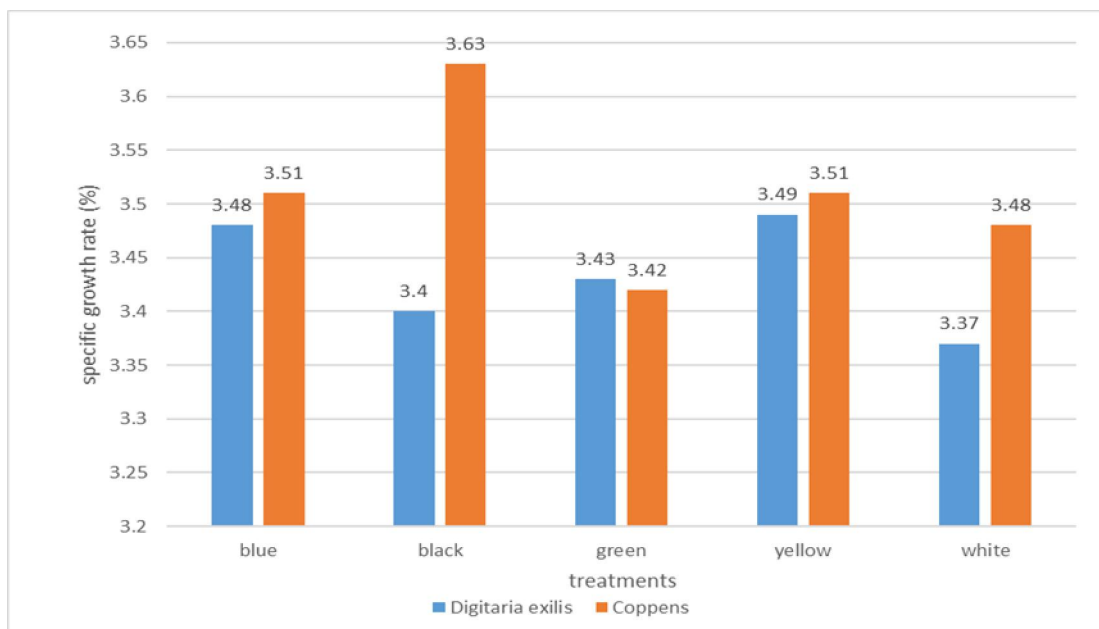
Figure 1: Summary of Specific Growth Rate derived after experimental period.
