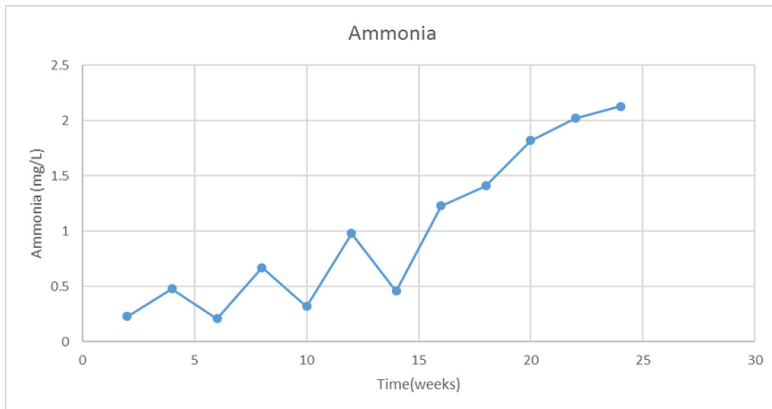
Figure 5: Average Ammonia Measured in all Treatments
