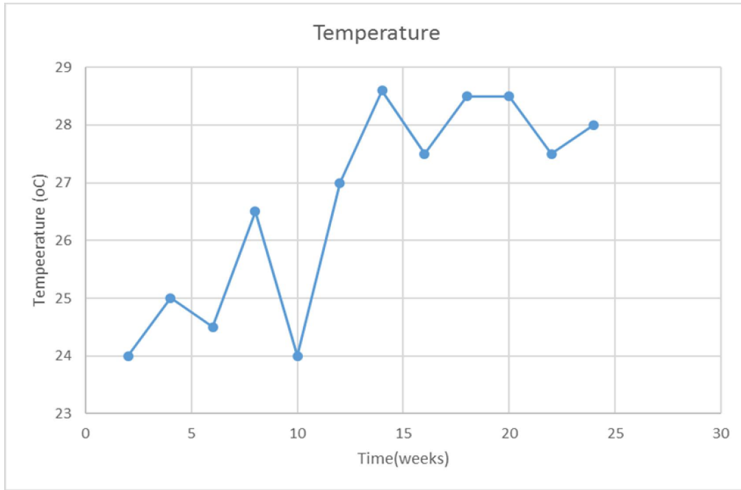
Figure 4: Average Temperatures Measured in all Treatments
