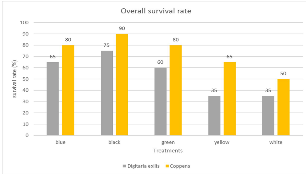
Figure 2: Overall Survival Rate of Heterobranchus bidorsalis derived in all Treatments during the Experimental Period.
