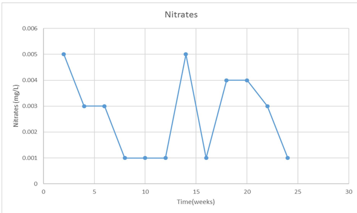
Figure 9: Average Nitrates Measured in all Treatments
