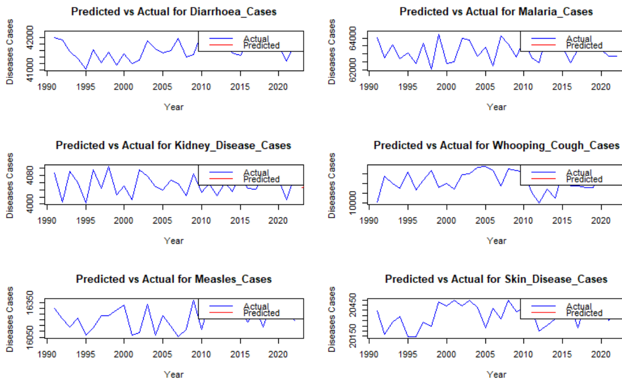
Figure 4.4: Prediction versus actual prevalence plot
