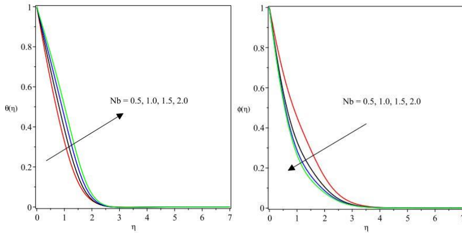
Fig. 16 temperature profiles versus Nb Fig. 17 concentration profiles versus Nb
