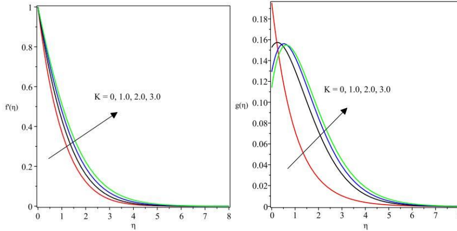
Fig. 2 velocity field versus K Fig. 3 microrotation profiles versus K
