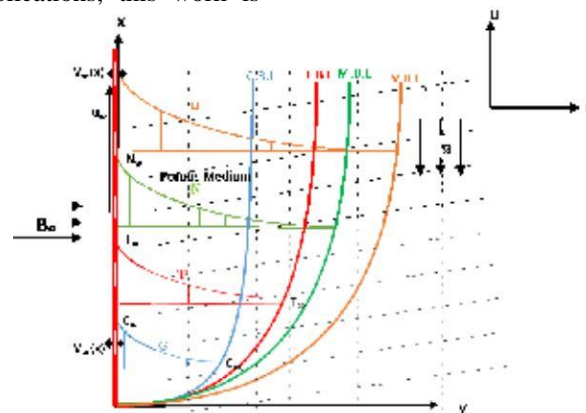
Fig. 1 Flow Geometry
