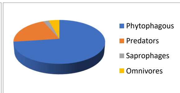
Fig.2. The guild structure of insect fauna
