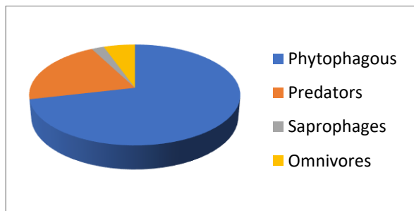
Fig.1. The guild structure of insect fauna
