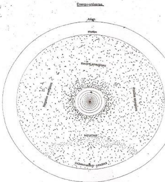
Energy particle has internal structure and having three kinds of basic elements proposed and named as Positive energies (PEONS), Negative energies (NEONS) and Neutral energies (NEUCONS); it is also another universe named as Energy-UNIVERSE having structure and properties exactly similar to the structure and properties resembling our Geo-UNIVERSE and Atomic-UNIVERSE.
