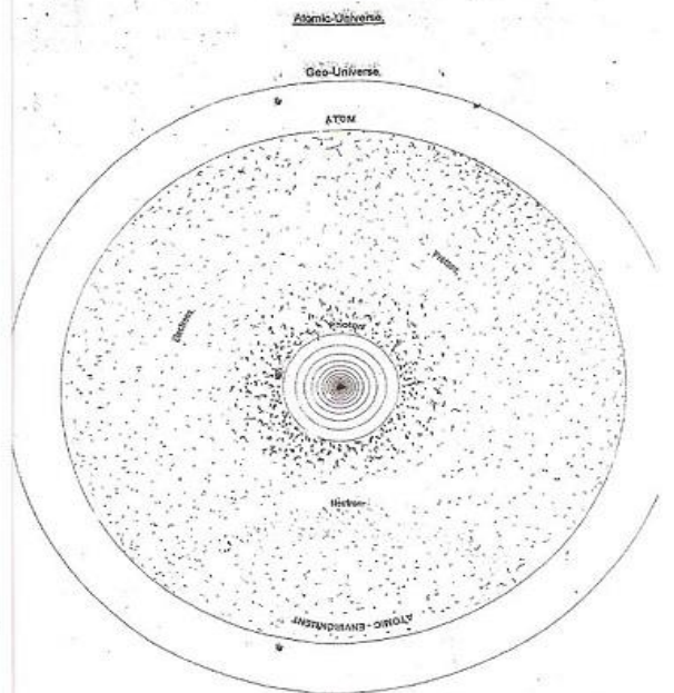
Atom is gigantic UNIVERSE having structure and properties exactly similar to the structure and properties resembling our Geo-UNIVERSE and Energy particle. Just like there are stars, planets, galaxies and life on the earth etc. present in the Geo-UNIVERSE; in the same way exactly similar stars, planets, galaxies and life on neutron's etc. may be present in the form of electrons, protons and neutrons in the atom.
