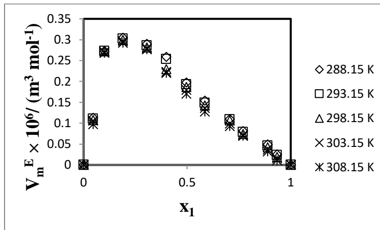
Figure 2 Excess molar volumes for tert-butyl methyl ether (1) + dipropyl amine (2) mixtures at different temperatures
