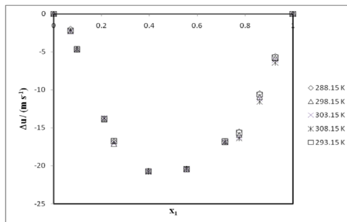
Figure 3 Deviations in speeds of sound \Delta u for tert-butyl methyl ether (1) + propyl amine (2) mixtures at different temperatures
