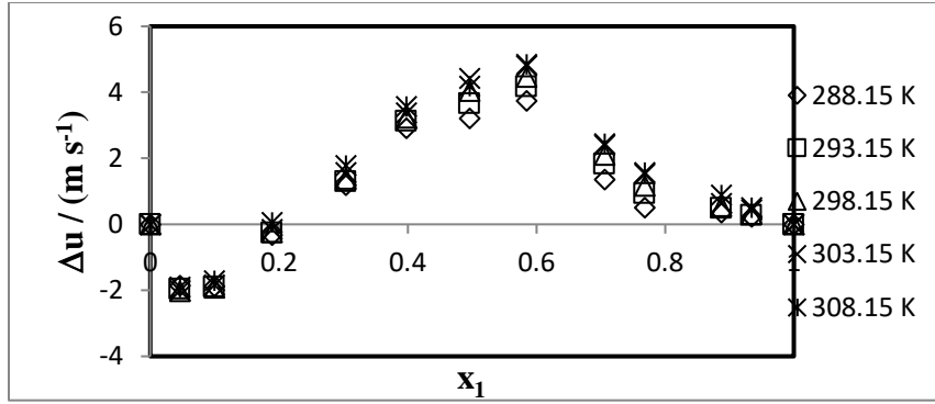
Figure 4 Deviations in speeds of sound \Delta u for tert-butyl methyl ether (1) + dipropyl amine (2) mixtures at different temperatures.
