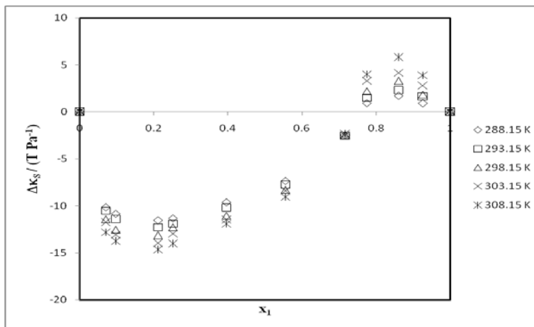
Figure 5 Deviations in isentropic compressibility \Delta \kappa_s for tert-butyl methyl ether (1) + propyl amine (2) mixtures at different temperatures.
