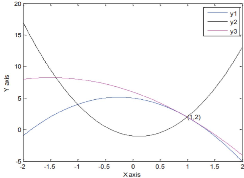
Fig. 1.2 Polynomials of Column vectors of Matrix B [Point of Concurrency is (1, 2) which is (1, L (B))]
