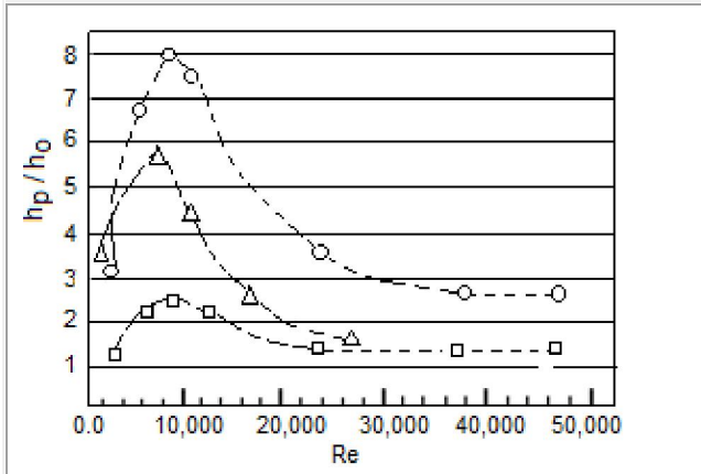
Fig. 12: Maximum enhancement values for upstream pulsation ( , 180 cm long & , 90 cm long) and downstream pulsation ( , 180 cm long). Counter flow using reciprocating pump, [8].
