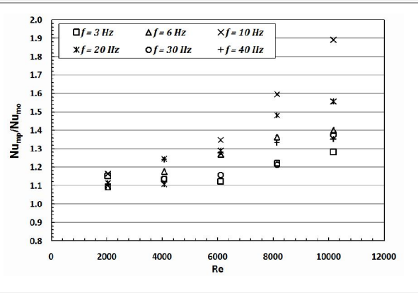
Fig. 7. Average Nusselt number ratio in the counter flow as a function of Reynolds number for different pulsation frequencies ( Th_i = 40\text{ }^\circ\text{C} )
