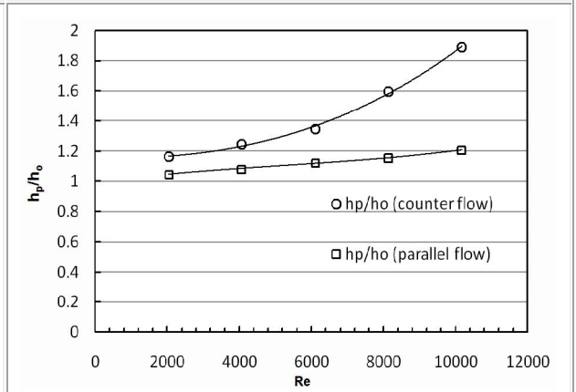
Fig. 13: Maximum enhancement values: downstream pulsation using ball valve;
