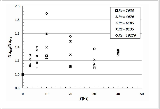
Fig. 9. Average Nusselt number ratio in the counter flow as a function of pulsation frequency for different Reynolds numbers ( Th_i = 40\text{ }^\circ\text{C} )
