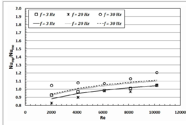
Fig. (16) Correlation of results of Nu_{mp}/Nu_{mo} for parallel flow ( T_{hi} = 70\text{ }^{\circ}\text{C} )
