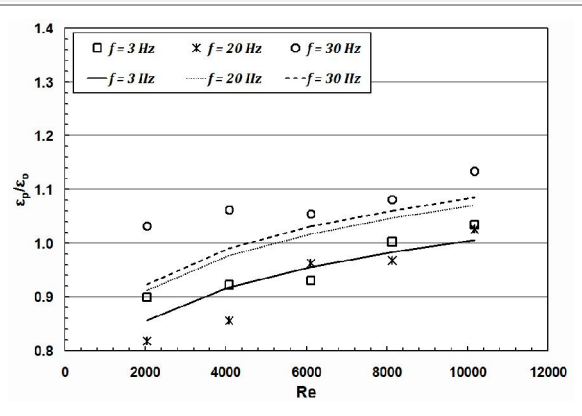
Fig. (17) Correlation of results of for parallel flow ( T_{hi} = 70\text{ }^{\circ}\text{C} )
