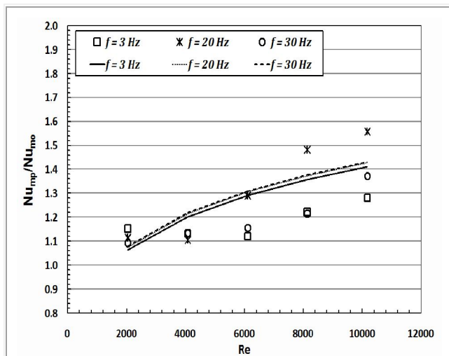
Fig. (14) Correlation of results of Nu_{mp}/Nu_{mo} for Counter flow ( T_{hi} = 40^\circ C )
