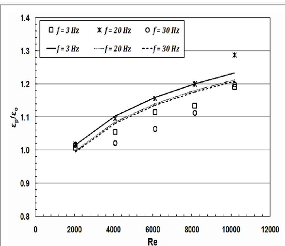
Fig. (15) Correlation of results of for Counter flow ( T_{hi} = 40^\circ C )
