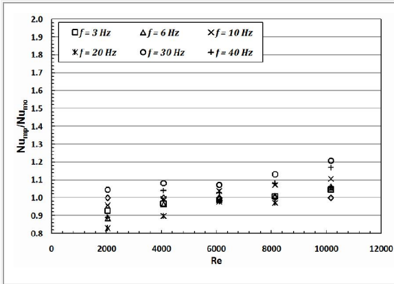
Fig. 6. Average Nusselt number ratio in the parallel flow as a function of Reynolds number for different pulsation frequencies ( Th_i = 70\text{ }^\circ\text{C} )
