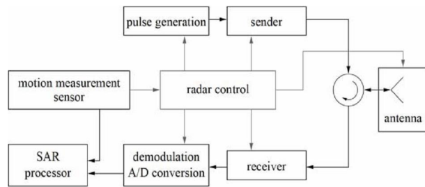
Figure 1. General structure of a SAR system
