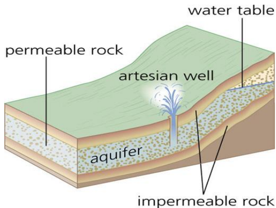
Figure 2. confined aquifers or artesian groundwater
