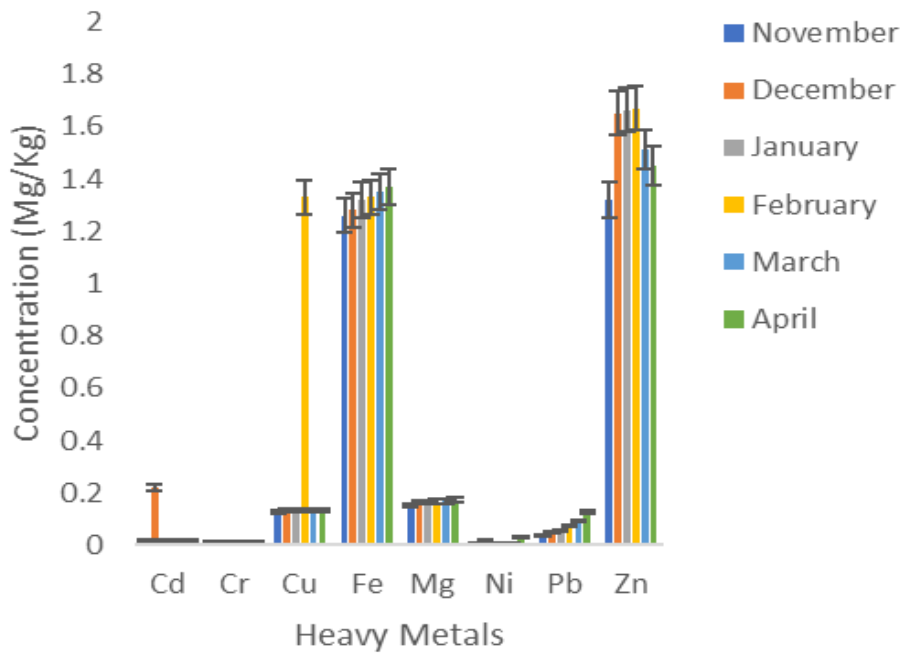
Fig. 2: Mean Heavy Metal Concentration (Mg/Kg) in the Tissue of Ethmalosa fimbata (Dry Season)
