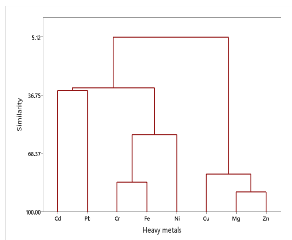
Fig 7: Wet season Dendrogram for Heavy Metals in Ethmalosa fimbriata
