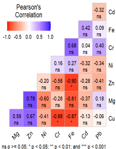
Fig. 6: Wet season Heavy metal correlation in the flesh of Ethmalosa fimbriata
