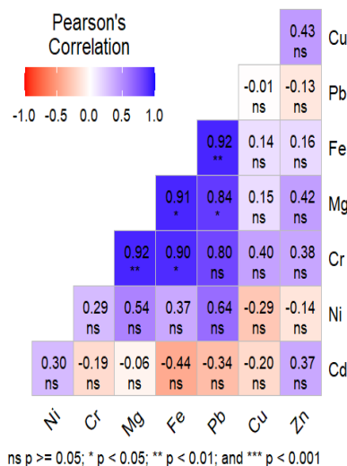
Fig. 4: Dry season Heavy metal correlation in the flesh of Ethmalosa fimbriata
