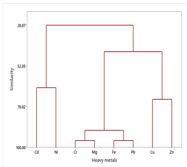
Fig 5: Dry season Dendrogram for Heavy Metals in Ethmalosa fimbriata
