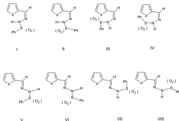
Figure 1. Various hypothetical conformations for compounds 1 and 2.
