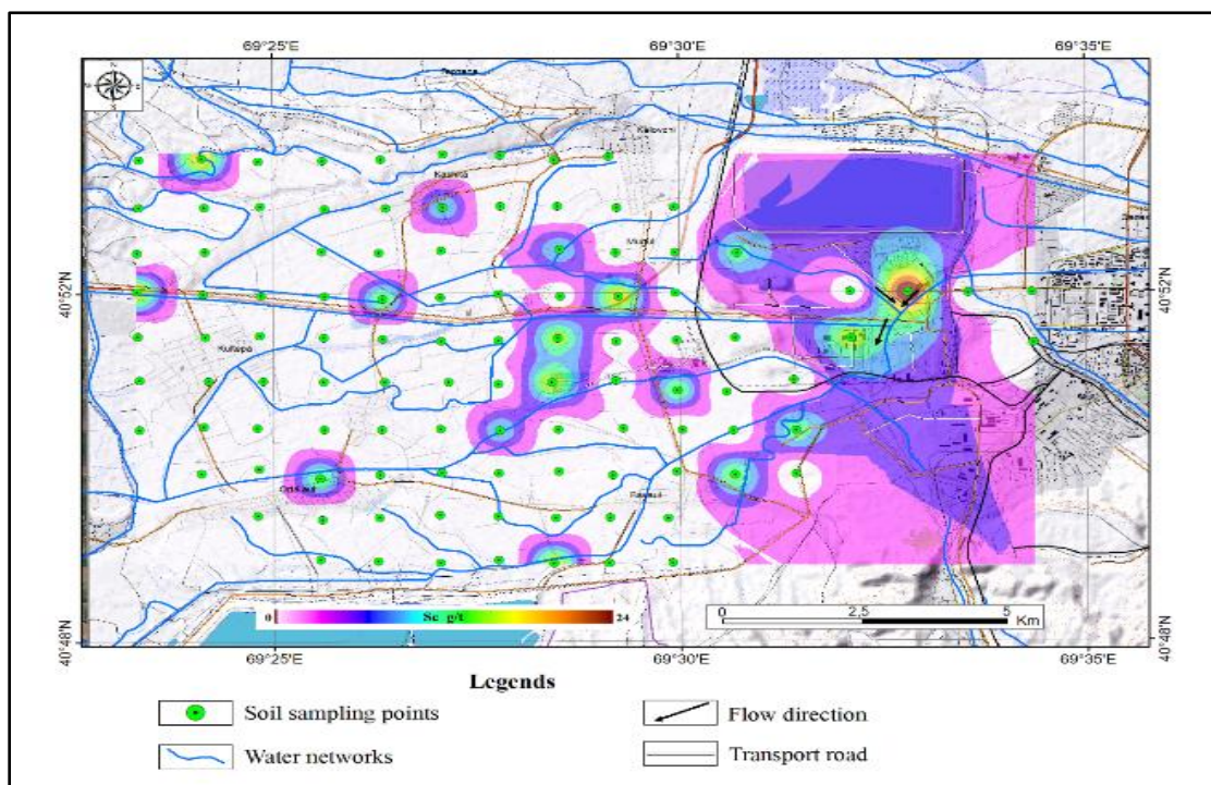
Fig.2. Distribution of the element scandium along the Gejigen network
