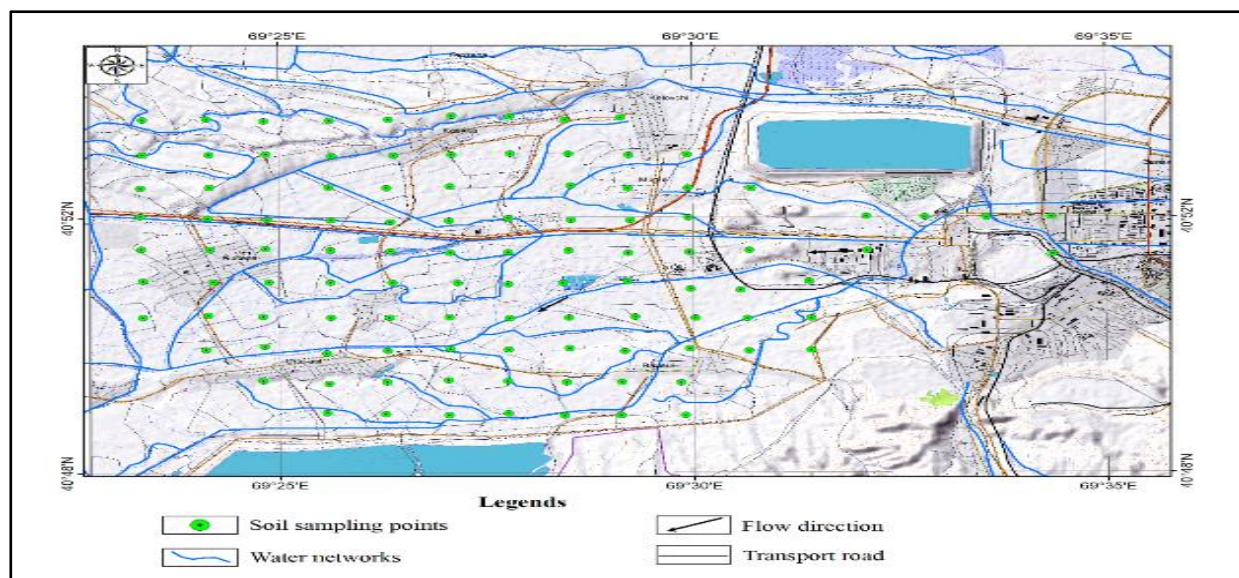
Fig.1. Soil sampling sites
