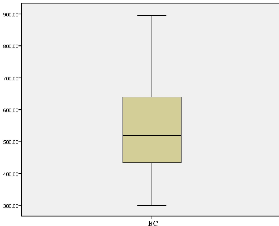
Figure 6- the box diagram of parameter EC
