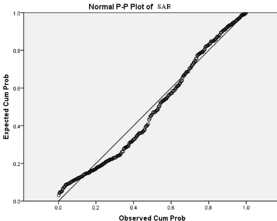
Figure 5-SAR data normality test
