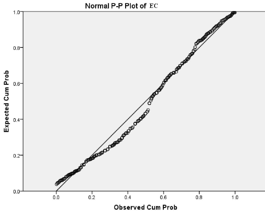
Figure 3- The EC data normality test
