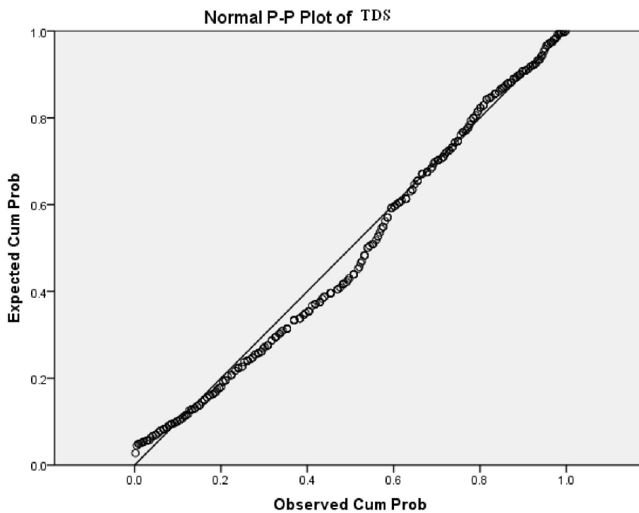
Figure 4- The TDS data normality test
