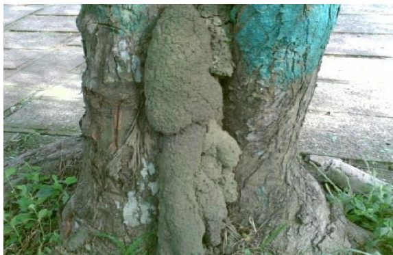
Fig. 7: Secondary pest termite attacking heartwood of live tree
