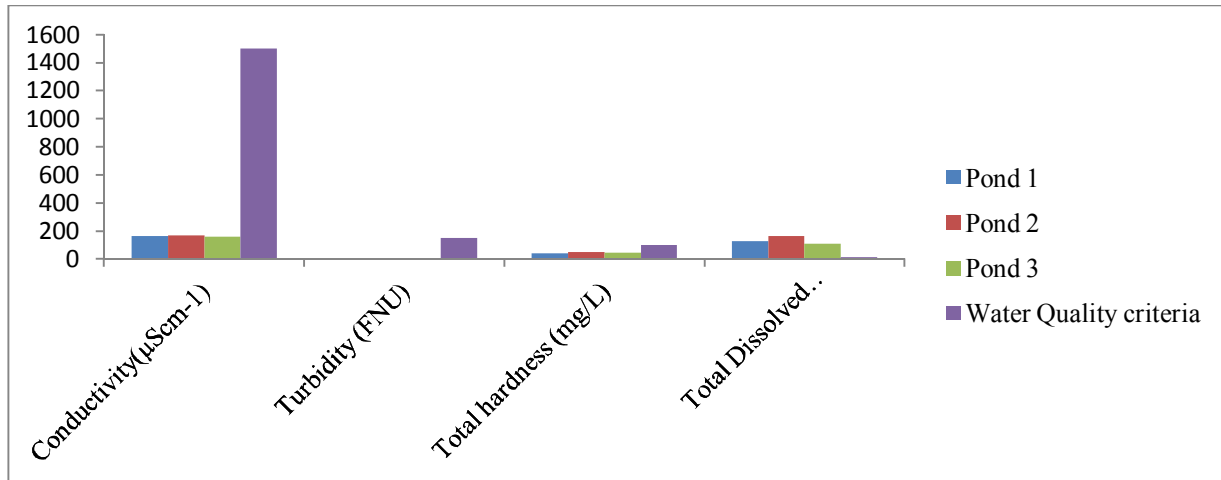
Fig.2: Conductivity ( \mu\text{Scm}^{-1} ), Turbidity (FNU), Total hardness (mg/l) and Total Dissolved Solids (mg/l) of the three ponds compared with Water quality criteria
