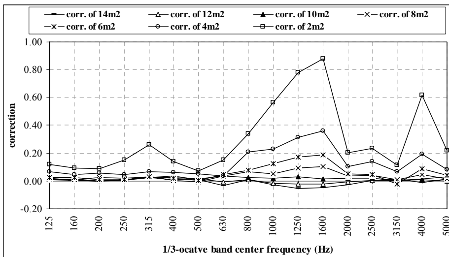
Fig.2c: absorption correction surface area for sponge material
