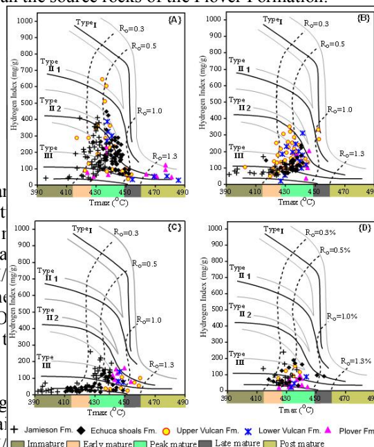
Figure 5.3: Cross-plots of Tmax versus Hydrogen Index (HI) defining kerogen types for source rocks samples from Central Caswell Sub-basin {A} Brewster-Ichthys Field {B} N & NE Caswell Sub-basin {C} Central Caswell Sub-basin {D} Brecknock -Buffon Trend.
