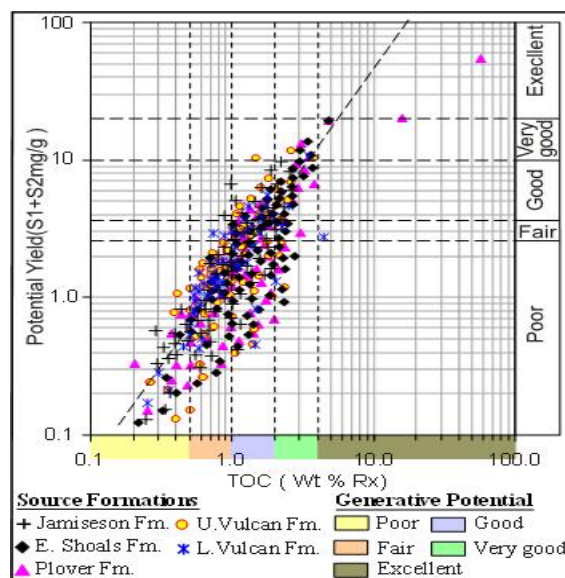
Figure 5.2: Plot of Potential Yield ( S_1+S_2 ) Versus TOC (iii) for Generation Potential of Source Rock samples from Caswell Sub-basin (Boundaries after Ghoria 1998)
