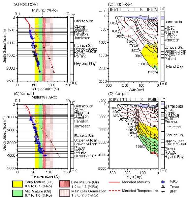
Figure 6.3: Thermal Maturity (calculated versus measured) and Geohistory Models of tow key wells; {(A & B) Rob Roy-1; (C & D) Yampi-1} in the Prudhoe Terrace
