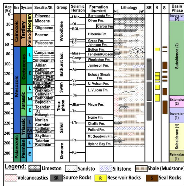
Figure 3.1: Stratigraphy of the Caswell Sub-basin showing Sequence Framework used for Geohistory Modelling (modified After Struckmeyer et al. 1998 and Blevin et al., 1998a)
