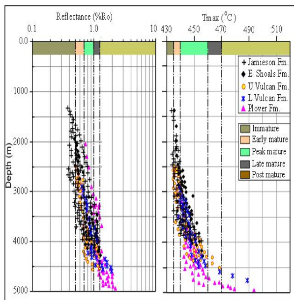
Figure 5.4: Maturity Depth Gradient based on Plot of Vitrinite Reflectance ( R_o ) and T_{max} versus Depth for the Source Rocks of Caswell Sub-basin
