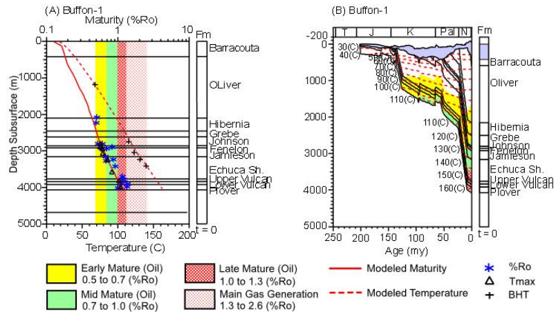
Figure 6.2: Thermal Maturity (calculated versus measured) and Geohistory Models of a key well of; (Buffon-1) in the Buffon–Brecknock Trend
