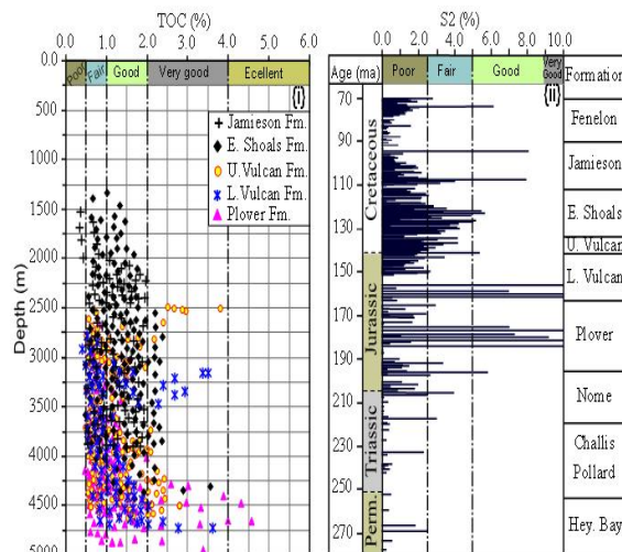
Figure 5.1: Plots of Depth (i) and Age (ii) Versus TOC and S_2 Values for Richness of Source Rock samples from Caswell Sub-basin
