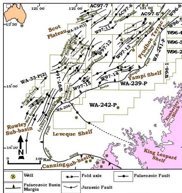
Figure 2.1: Browse Basin Map Showing Generalized Structural Elements and Trends (Modified after Allen et al. 1978)
