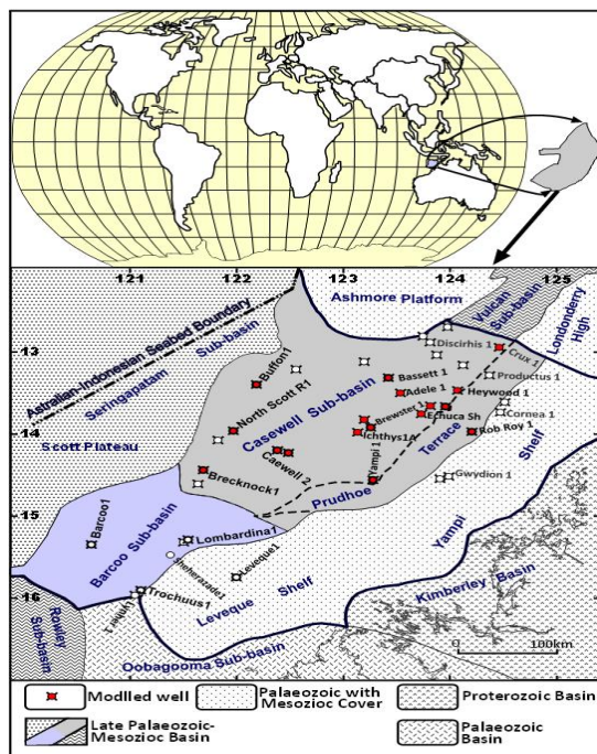
Figure 1.1: Location Map of the Caswell Sub-basin showing the modeled wells
