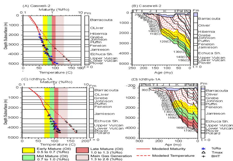
Figure 6.1: Thermal Maturity (calculated versus measured) and Geohistory Models of tow key wells; {(A & B) Caswell-2; (C & D) Ichthys-1A} in the Central Caswell Sub-basin
