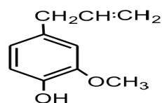
Eugenol
