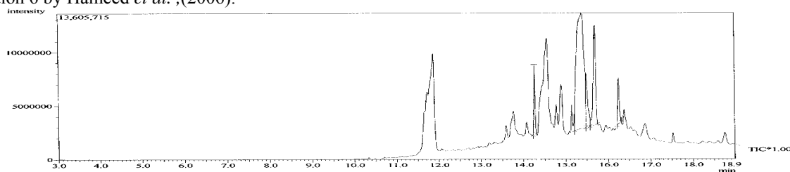
Figure 1: GC/MS chromatogram of equilibrium concentration atrazine after adsorption onto SS/A/5gL -1 sorbent (Carrier gas-Helium 100.2kpa, Column temperature -60°C, Injection temperature-250°C, Injection volume—1µL, Flow rate-1.61mL/min, Injection method- split, Linear velocity- 43.6cm/sec.)
