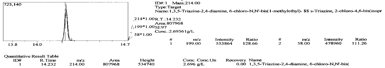
Figure 2: GC/MS chromatogram, quantitative measurement and spectral information of equilibrium phase atrazine after adsorption onto SS/A/5gL -1 sorbent
