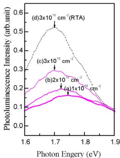
Figure 6. PL spectra of the Si + -implanted 400-nm-thick SiO 2 film grown on crystal Si at a fluence of (a) 1x10 16 ions/cm 2 , (b) 2x10 16 ions/cm 2 , and (c) 3x10 16 ions/cm 2 after dry-N 2 CTA for 12 hours at 1150°C and at a fluence of (d) 3x10 16 ions/cm 2 after dry-N 2 isothermal RTA for 20 seconds.
