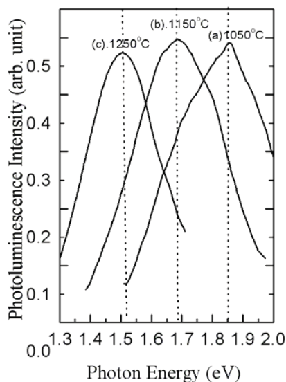
Figure 2. PL spectra of the \text{Si}^+ -implanted 400-nm-thick \text{SiO}_2 film grown on crystal Si at a fluence of 3 \times 10^{16} ions/ \text{cm}^2 after dry- \text{N}_2 RTA for 20 seconds at (a) 1050°C, (b) 1150°C, and (c) 1250°C.
