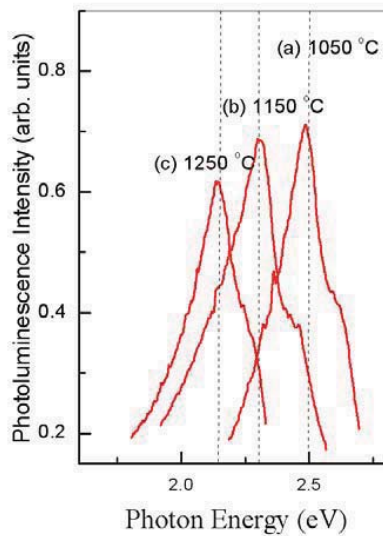
Figure 1. PL spectra of the \text{Si}^+ -implanted 400-nm-thick \text{SiO}_2 film grown on crystal Si at a fluence of 1 \times 10^{16} ions/ \text{cm}^2 after dry- \text{N}_2 RTA for 5 seconds at (a) 1050°C, (b) 1150°C, and (c) 1250°C.
