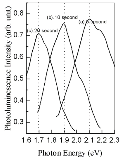
Figure 3. The PL spectra of the \text{Si}^+ -implanted 400-nm-thick \text{SiO}_2 film grown on crystal Si at a fluence of 3 \times 10^{16} ions/ \text{cm}^2 after dry- \text{N}_2 RTA at 1150 °C for (a) 5 seconds, (b) 10 seconds, and (c) 20 seconds.
