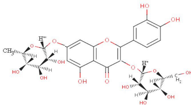
Compound (B)
