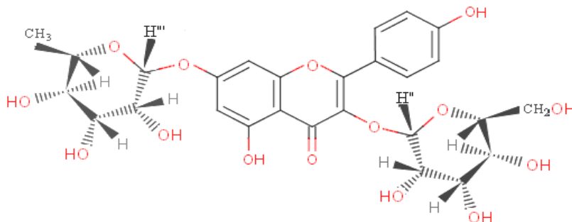
Compound (A)
