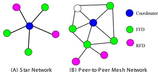
Figure 5. ZigBee Network Topology.
