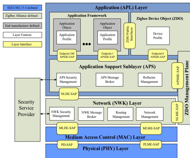
Figure 4. ZigBee stack.
