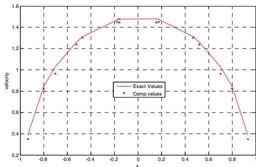
Figure 4: Comparison of computed and analytical velocity distributions over the surface of a sphere using 96 boundary elements
