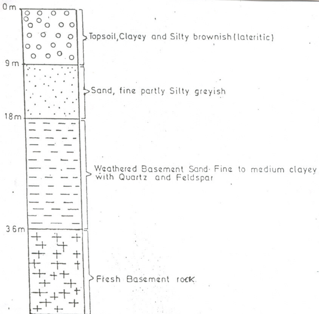
Fig. 5: Geological Well-log obtained by Preussag Nig. Ltd. at Jama'a Kubanni (after Olugbemiro, 1985)
