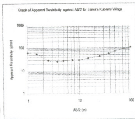
Fig. 3: VES 2 Curve for the Alternative Equipment
