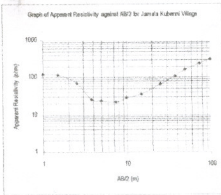
Fig. 2: VES 1 Curve for the Terrameter, T
