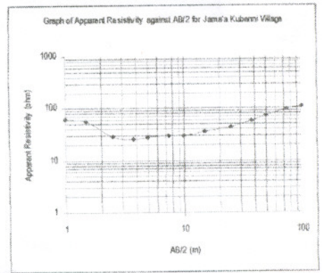
Fig. 4: VES 3 Curve for the Older Equipment
