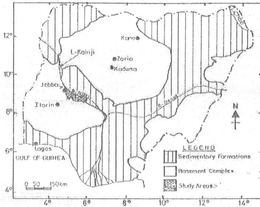
FIG. 1 FIG. 1: SIMPLIFIED GEOLOGICAL MAP OF NIGERIA SHOWING THE TWO LOCAL GOVERNMENT AREAS STUDIED (Courtesy of GSN)
