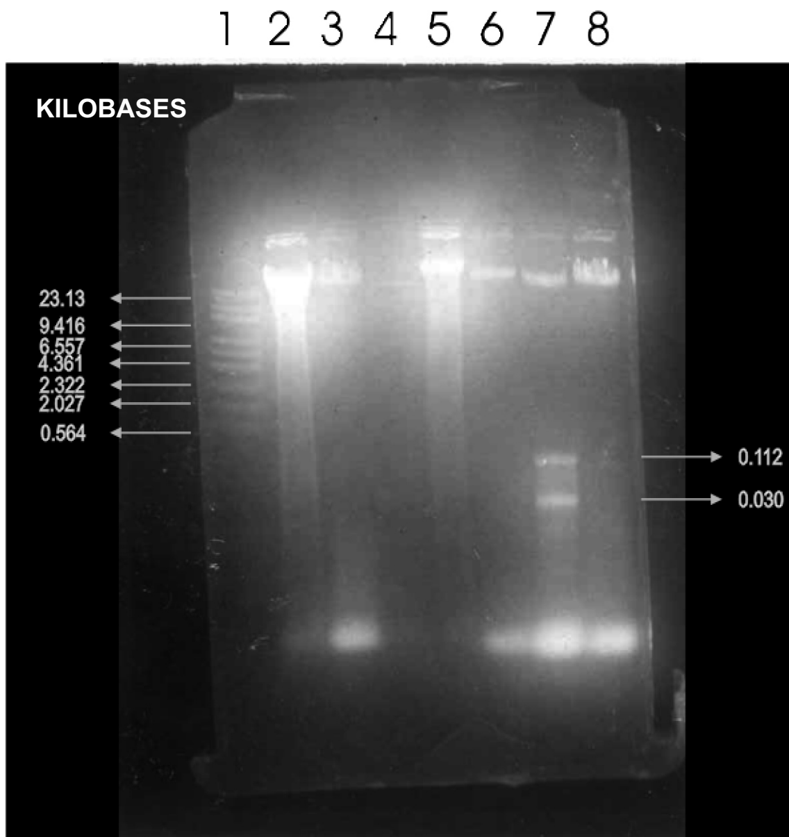
Plate 3: Agarose gel electrophoresis plate showing plasmid DNA isolated from Pseudomonas aeruginosa using the protocol of Birnboim and Doly (1979). Lanes: 1, \lambda DNA Hind 111 digested (marker); 2, Proteus mirabilis ; 3, Proteus mirabilis ; 4, Escherichia coli ; 5, Escherichia coli ; 6, Escherichia coli ; 7, Pseudomonas aeruginosa ; 8, Proteus mirabilis .
