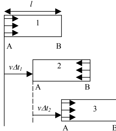
Figure 5. The demonstration of the Lorentz contraction. In a moving box at the velocity v of right direction, a light ray emits from mirror A and travels to mirror B (length AB) then reflects back to mirror A (length BA).
