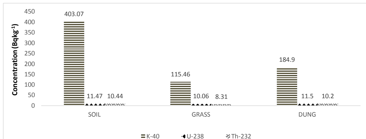
Fig 2: Mean distribution of radionuclides in all samples
