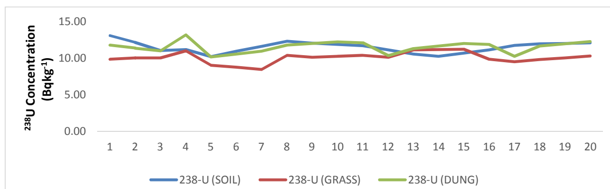
Fig 5: Distribution of 238 U concentrations in soil, grass, and dung.
