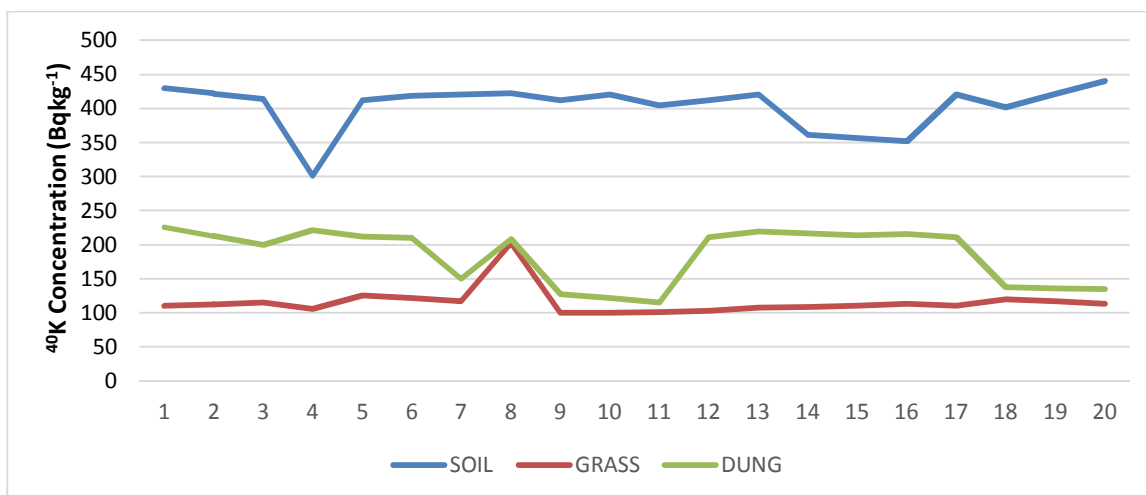
Fig 4: Distribution of 40 K concentrations in soil, grass, and dung.
