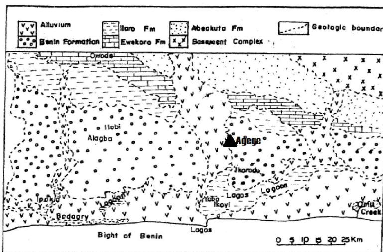
Figure 1: Geological Map of Lagos State showing Agege (the study area) 16 .
