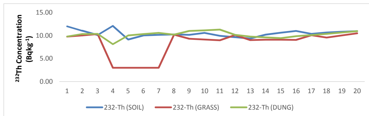
Fig 5: Distribution of 232 Th concentrations in soil, grass, and dung.
