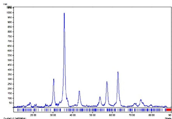
Figure 5. XRD pattern of Fe 3 O 4 nanoparticles
