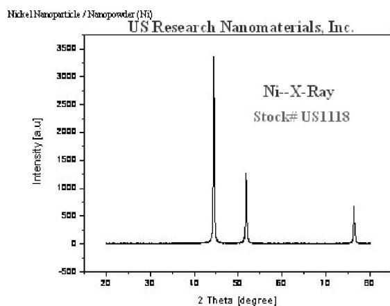
Figure.7. XRD pattern of Ni nanoparticles
