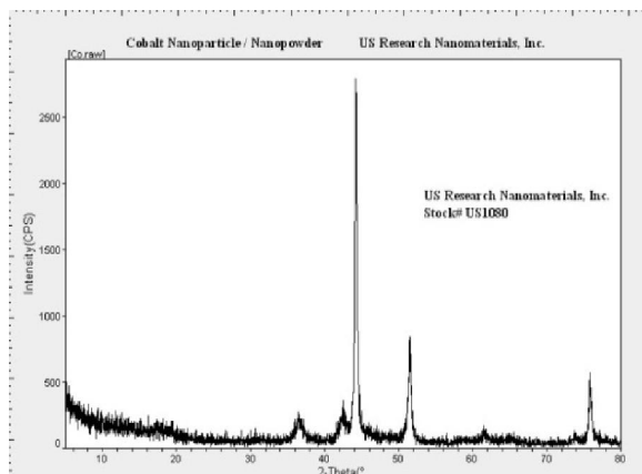
Figure.6. XRD pattern of Co nanoparticles
