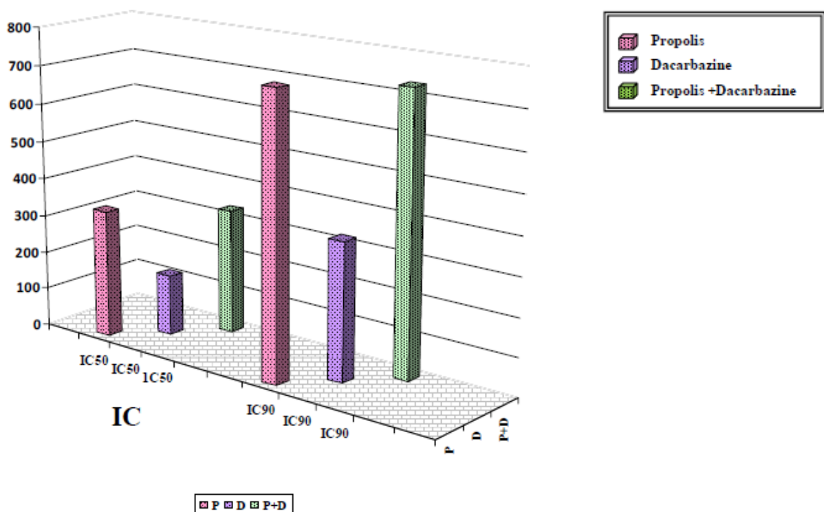
Fig ( 9 ) : Effects of Different concentrations of Treatment with Propolis ,Dacarbazine, and The Dual Treatment with Propolis and Dacarbazine on the IC50 and IC90 values of liver cancer cells of the lines HepG 2 after 48 h .
