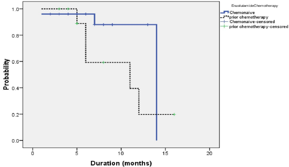
Figure (6) Overall Survival In Relation to Previous Chemotherapy
