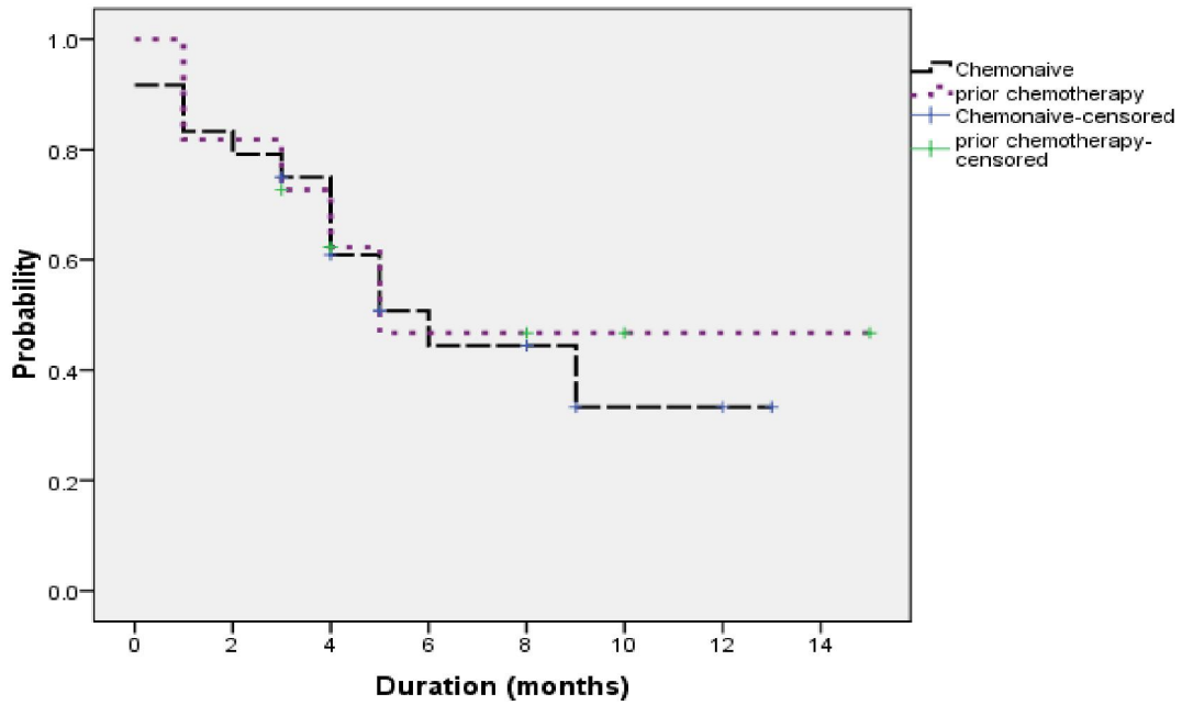
Figure (2) Progression Free Survival In Relation to Previous Chemotherapy
