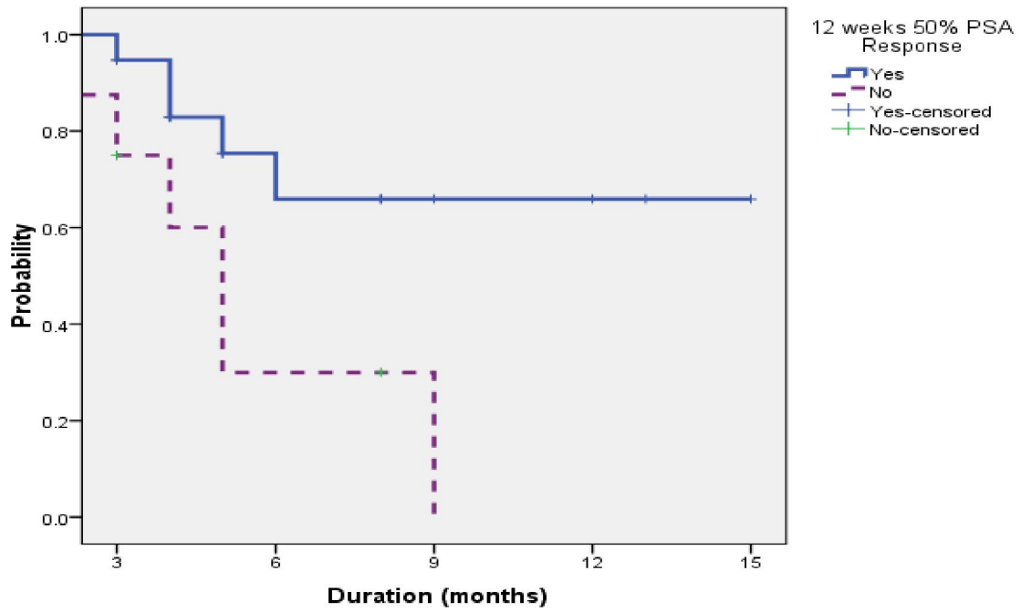
Figure (4) Progression Free Survival In Relation to PSA Response at 12 Weeks
