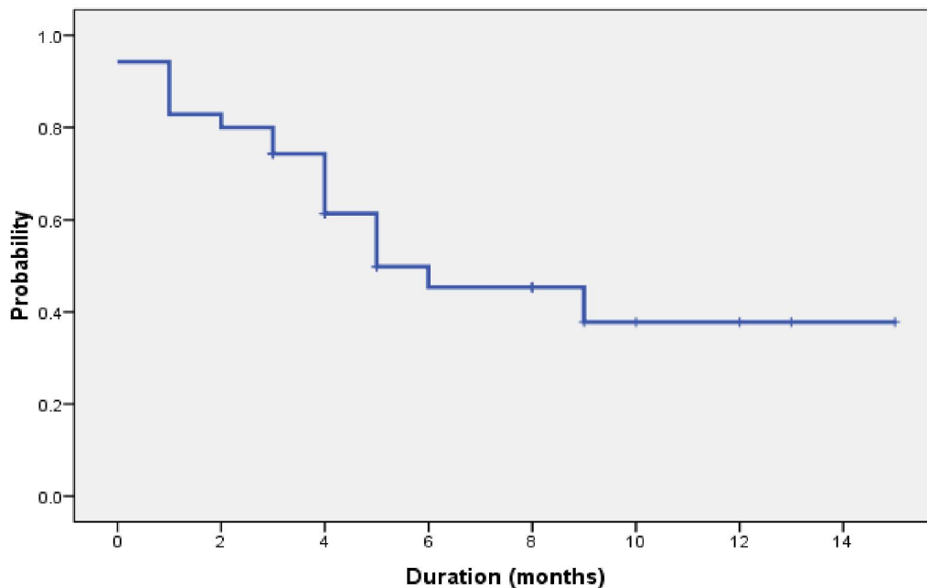
Figure (1) Progression Free Survival
