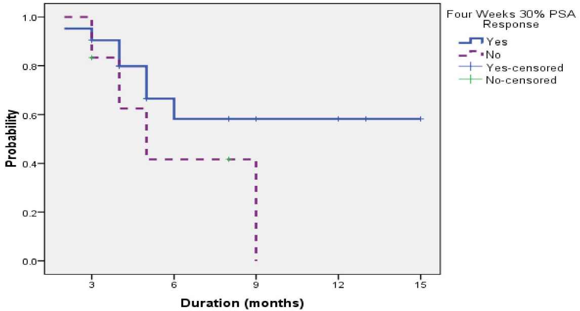
Figure (3) Progression Free Survival In Relation to PSA Response at Four weeks
