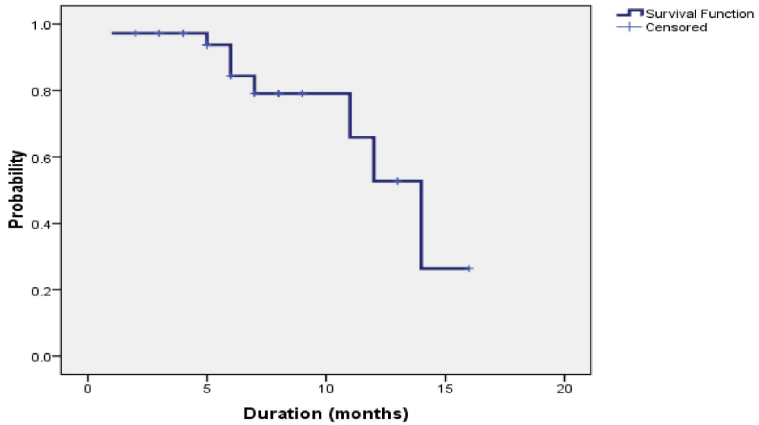
Figure (5) Overall Survival Since Enzalutamide Treatment
