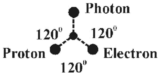
(Neutrino Oscillation)
