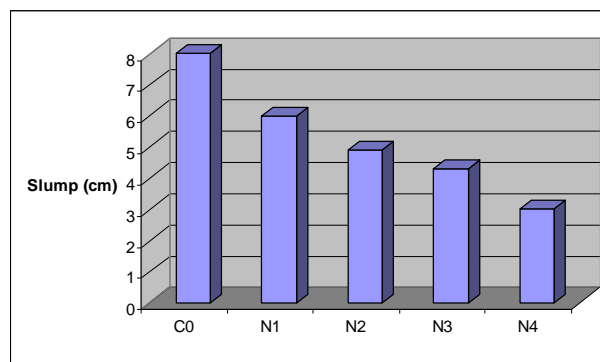
Figure 1. Particle size effects of nano- Fe 2 O 3 on workability of concrete. N1,N2,N3 and N4 are the series N blended concrete with 0.5, 1.0, 1.5 and 2.0 percent of nano- Fe 2 O 3 particles, respectively.
