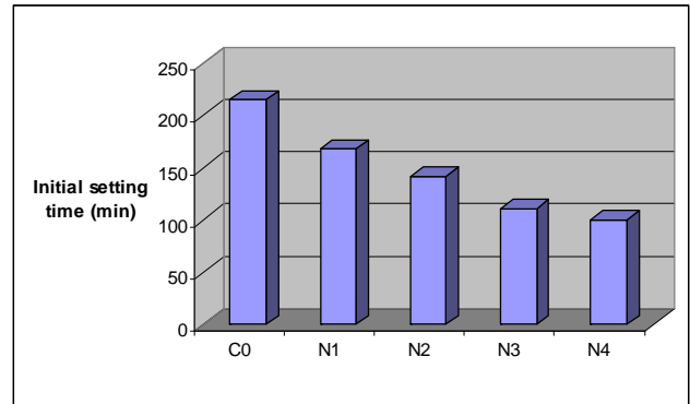
Figure 1. Influence of nano-Al 2 O 3 particles on the initial setting time of cement paste.
