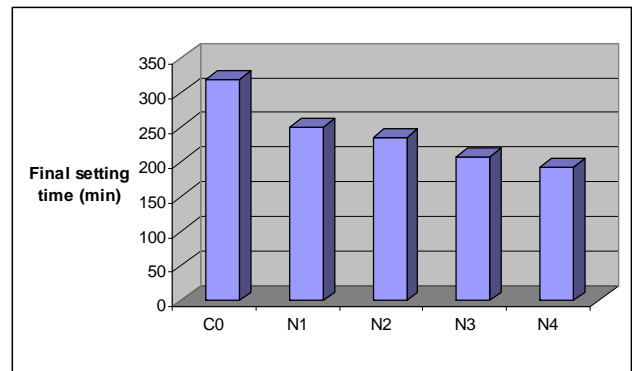
Figure 2. Figure 1. Influence of nano-Al 2 O 3 particles on the initial setting time of cement paste.
