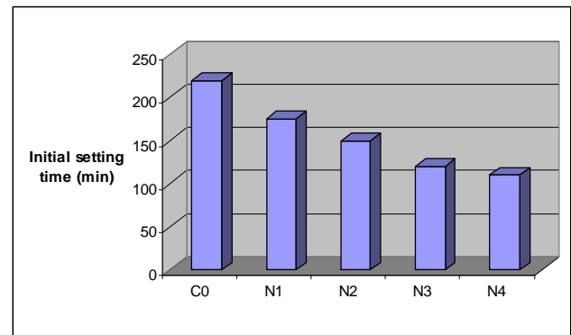
Figure 1. Influence of nano- Fe 2 O 3 particles on the initial setting time of cement paste.
