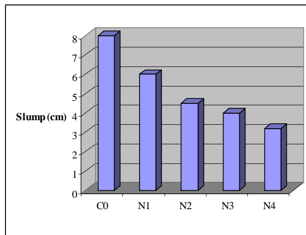
Figure 1. Particle size effects of nano-SiO 2 on workability of concrete. N1,N2,N3 and N4 are the series N blended concrete with 0.5, 1.0, 1.5 and 2.0 percent of nano-SiO 2 particles, respectively.
