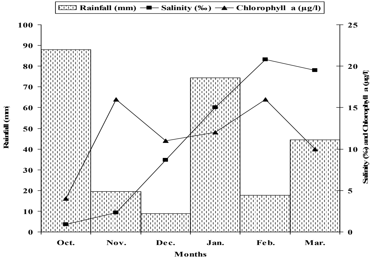
Fig. 2: Monthly variations in Rainfall, Salinity and Chlorophyll a at the Badagry creek (October, 2007 – March, 2008).
