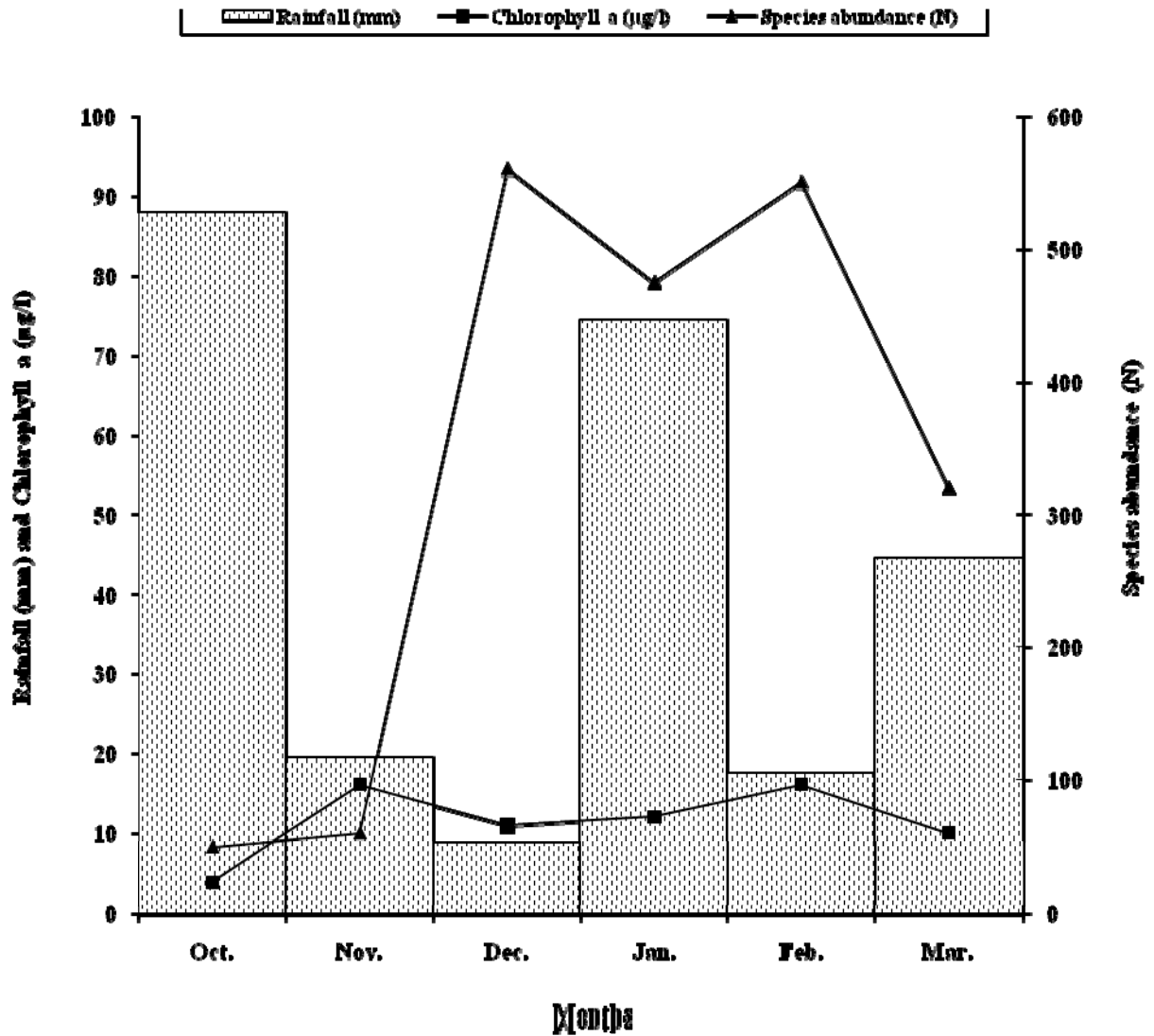
Fig. 3: Monthly variations in Rainfall, Chlorophyll a and Species abundance at the Badagry creek (October, 2007 – March, 2008).
