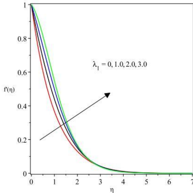
Fig. 8 velocity profiles profiles versus \lambda_1 Fig. 9 velocity profiles profiles versus \lambda_2
