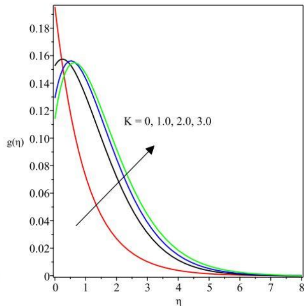
Fig. 2 velocity field versus K Fig. 3 microrotation profiles versus K
