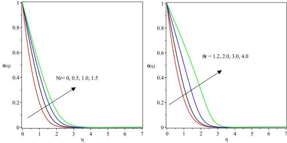
Fig. 12 temperature profiles versus Nr Fig. 13 temperature field versus \theta_r
