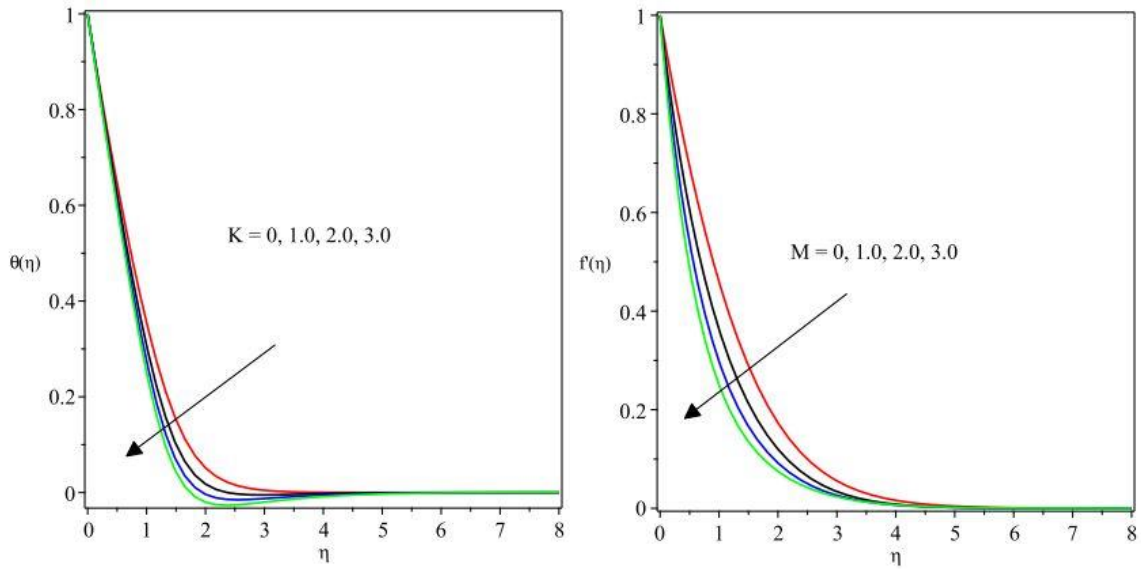
Fig. 4 temperature profiles versus K Fig. 5 velocity profiles versus M
