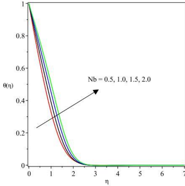
Fig. 16 temperature profiles versus Nb Fig. 17 concentration profiles versus Nb
