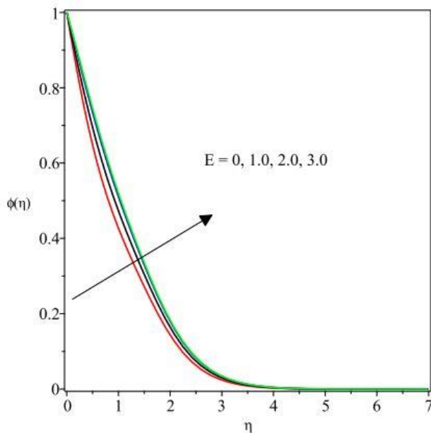
Fig. 18 concentration profiles versus E Fig. 19 concentration profiles versus Sc
