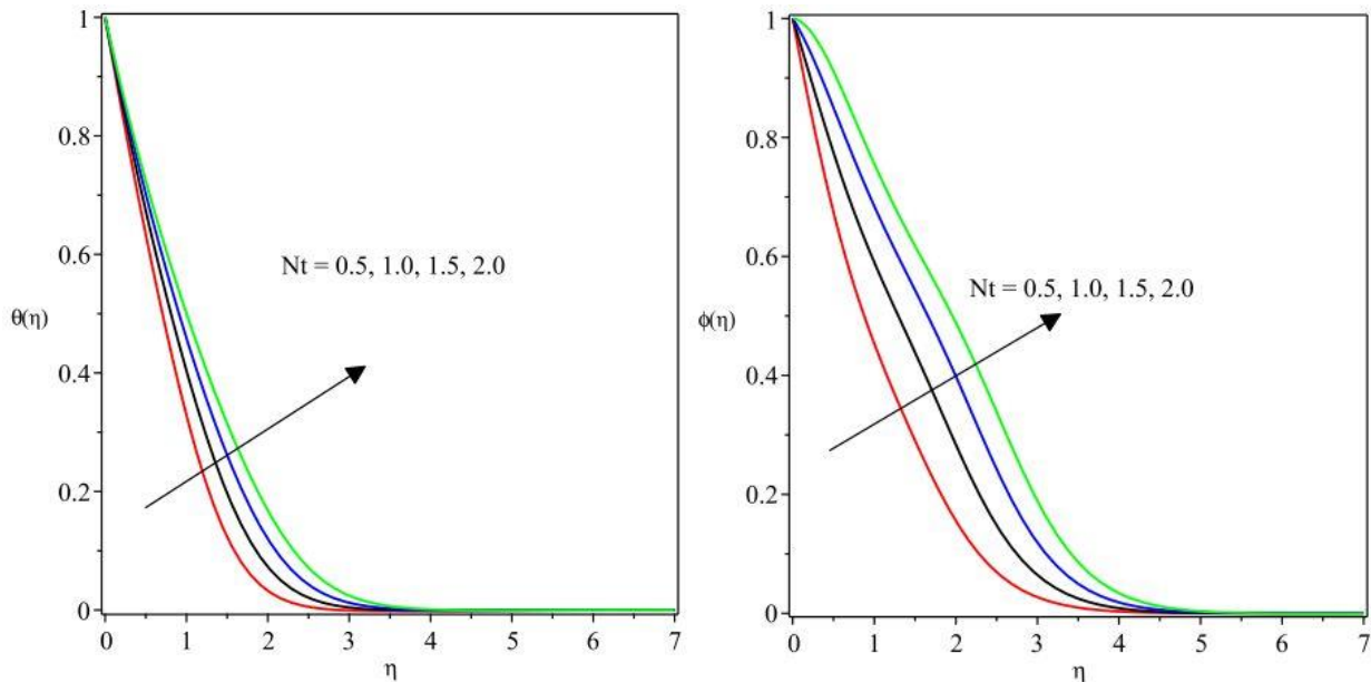
Fig. 14 temperature profiles versus Nt Fig. 15 concentration profiles versus Nt
