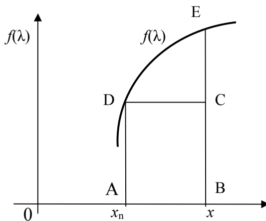
Figure 1.2: Approximating the area by the rectangle ABCD
